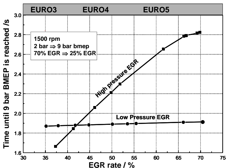
Fig. 18: Load Change for Different EGR-Rates and EGR-Split
